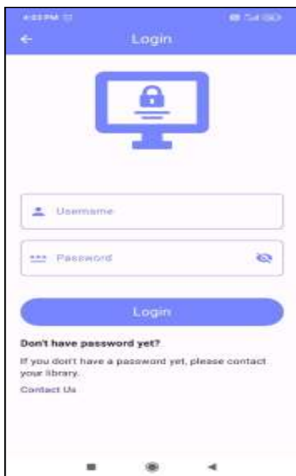
Figure 3: User Login
