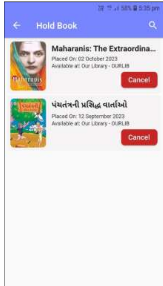
Figure 6: Hold Book
